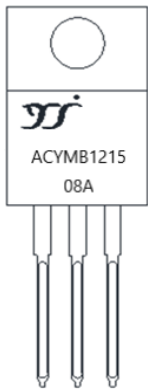
(TO-220AB-1 Package)
