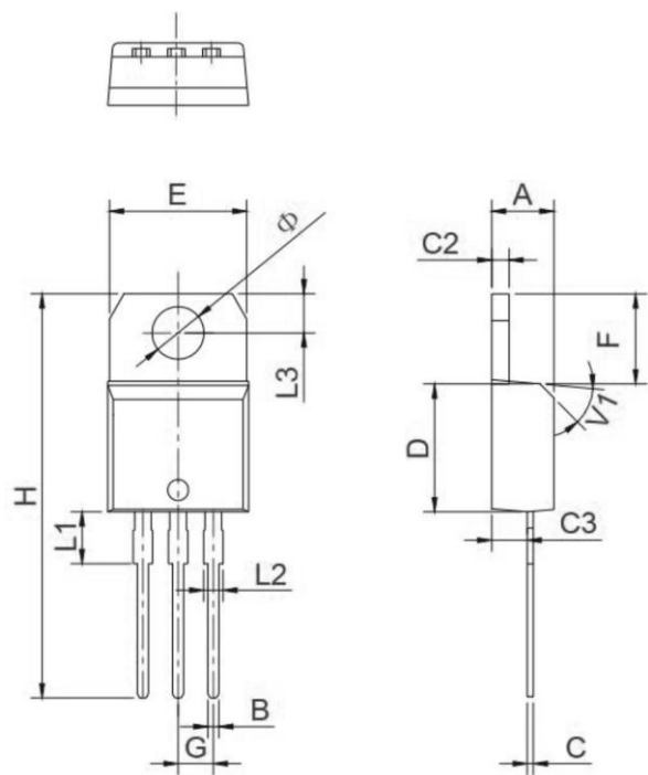
TO-220AB-1
