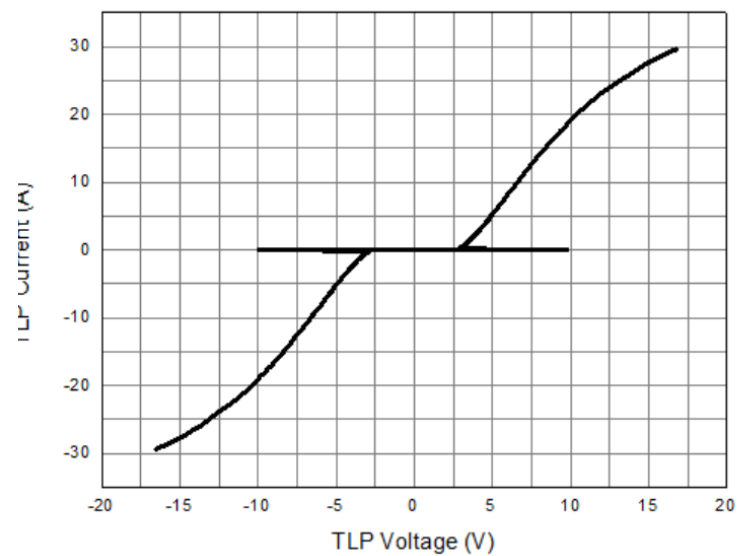
Fig.4: Transmission Line Pulsing TLP Plot
